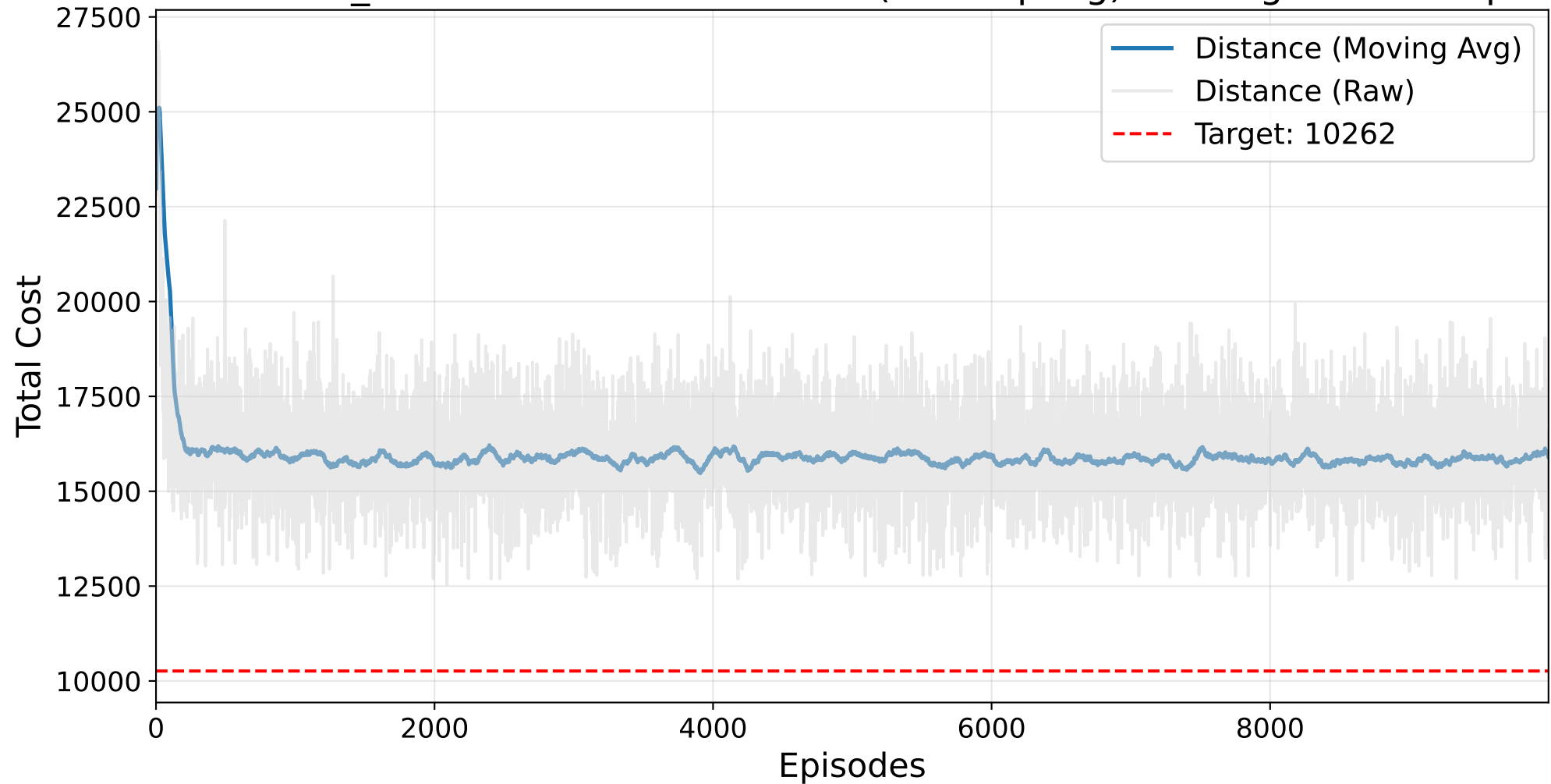
Final NO_MASK Masked AutoRL-SOP (Resampling) Training - ft53.3.sop
